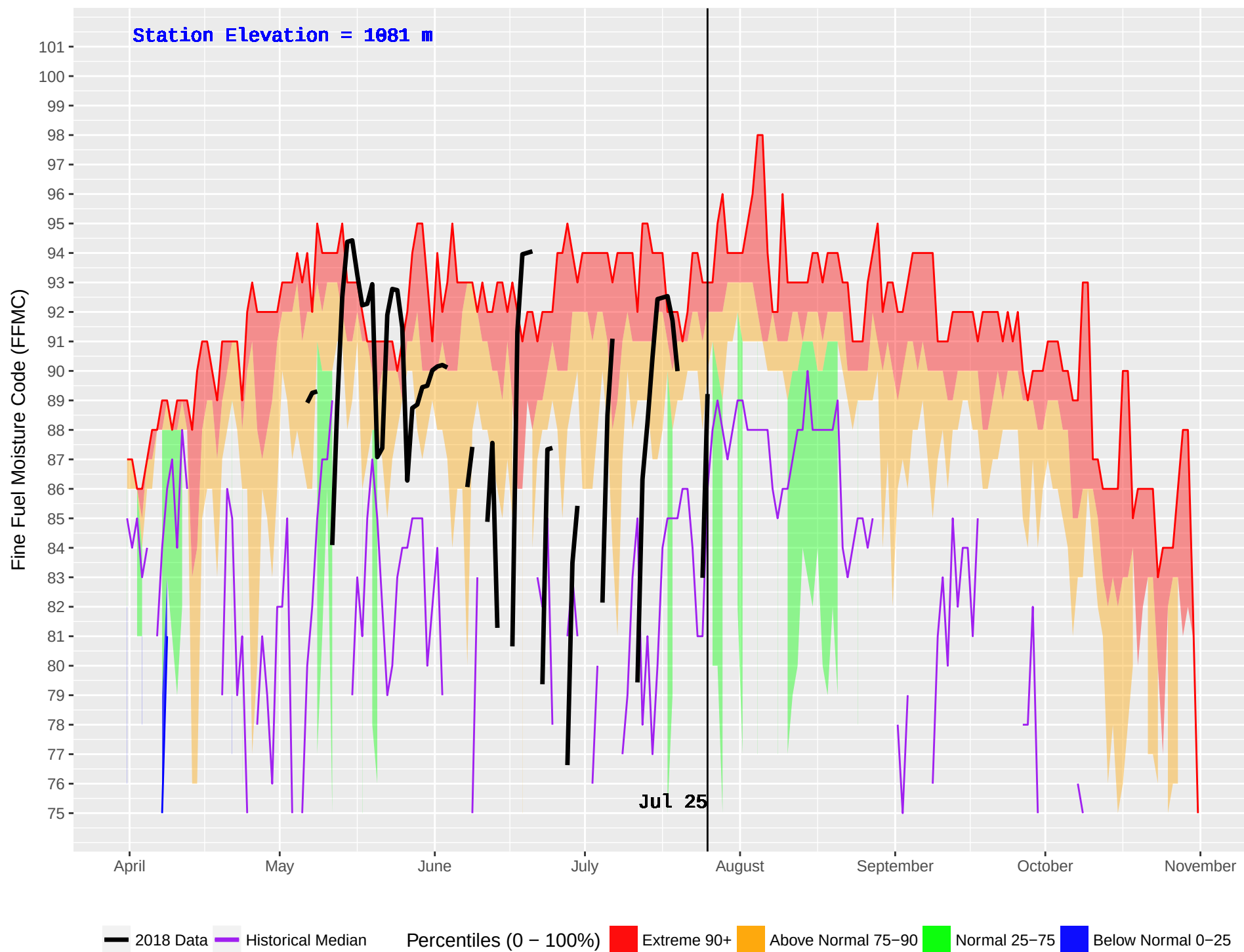
GAVIN (227) : Historical (1981–2016) and Current (2018) Noon Fine Fuel Moisture Code (FFMC)
