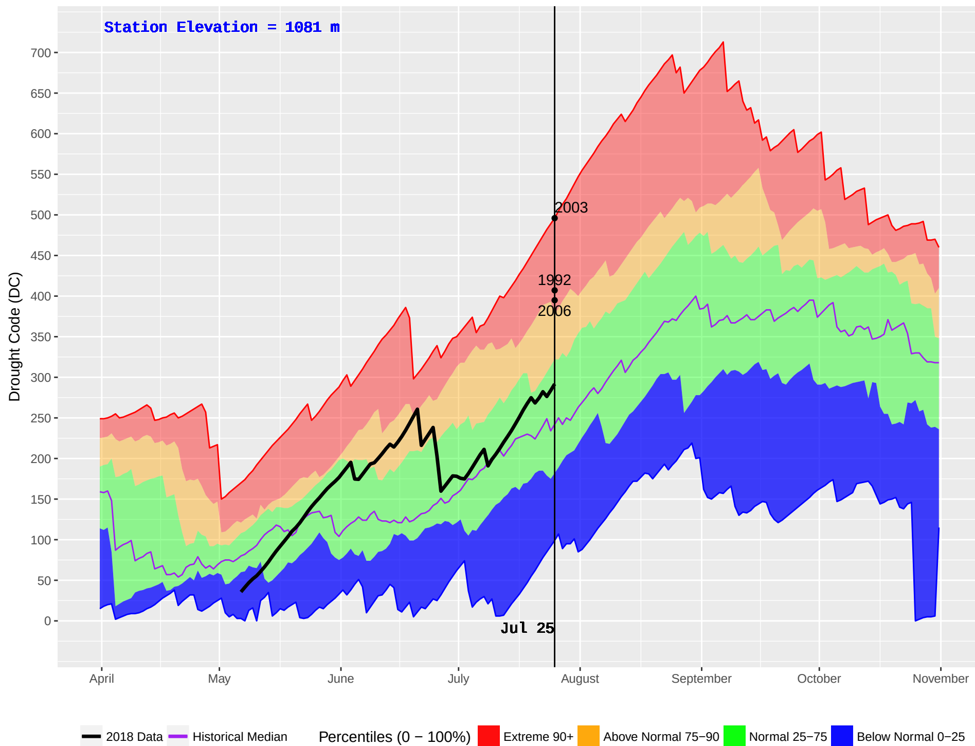
GAVIN (227) : Historical (1981–2016) and Current (2018) Noon Drought Code (DC)
