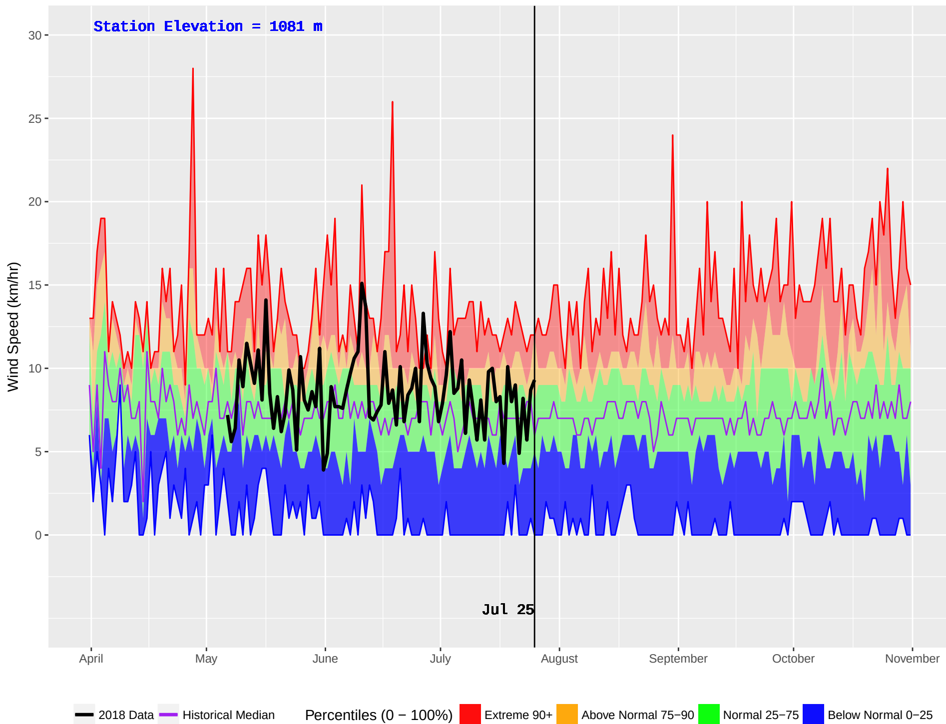
GAVIN (227) : Historical (1981–2016) and Current (2018) Noon Wind Speed
